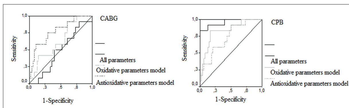
Figure 4. ROC curves of the discriminatory ability of selected parameters regarding postoperative complications in all CABG patients, and in the CPB group.
